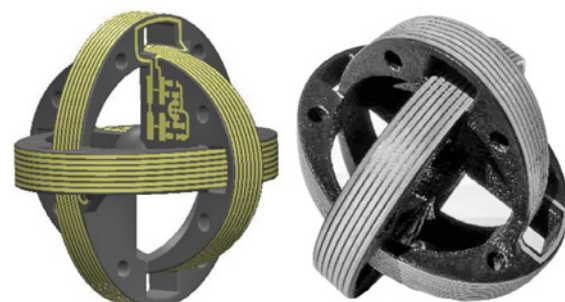
3D-MID circuitry for omni-directional inductive wireless power transfer
