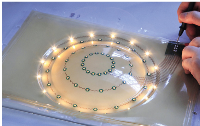
Thermoformed 3D-MID with a TPU substrate laminated to PC or PMMA
