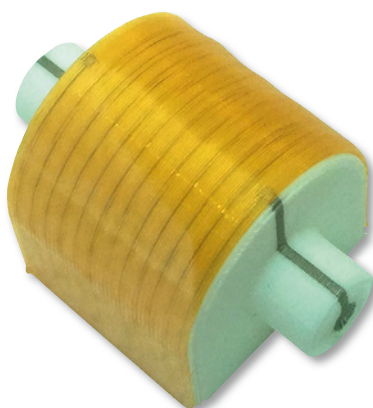
Hyb-Man project 3D printed PLA heater with printed circuit tracks
