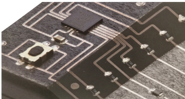
3D MID with printed nanoscale silver ink circuit tracks
